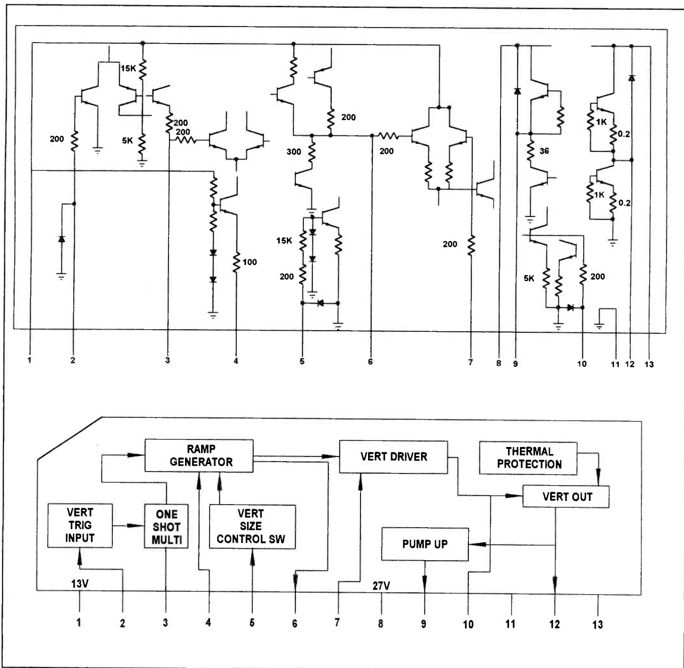
Figure 4. The LA78XX series of vertical output ICs (of which IC451 in the Quasar TS2523EK is an example) is used in a number of TV sets. The exact part number depends on the screen size, but the pinout remains unchanged. This particular one reproduces the insides of an LA78388 from the perspective of a Sharp engineer.
