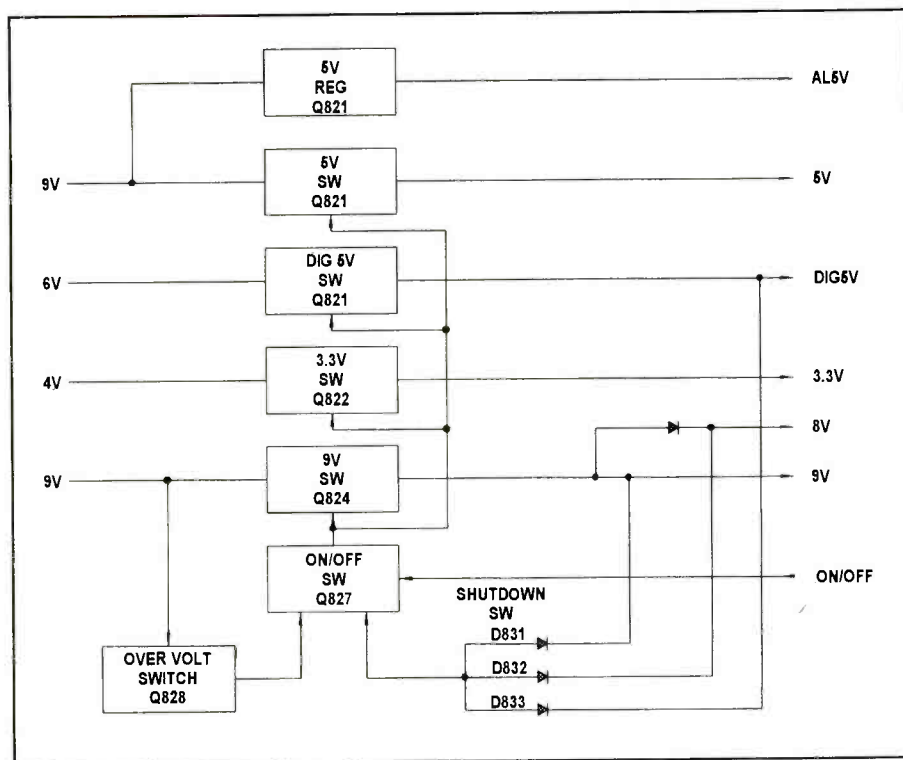
Figure 2. Block diagram of the secondary voltage outputs in the DVD 400/420.
