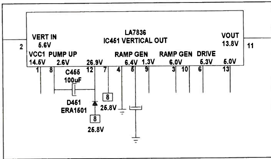
Figure 2. There was no sign of B+ at pins 7 and 12 of IC 451 in a Quasar model TS2523EK, which exhibited the symptom of failure of the vertical deflection.
